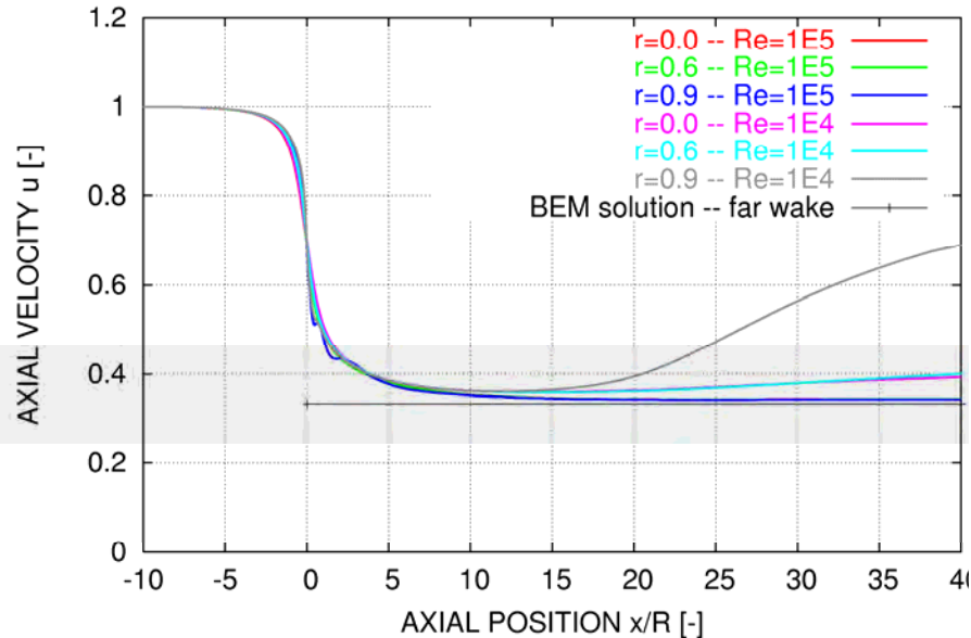
AD simulations -- constant loading CT=0.89
