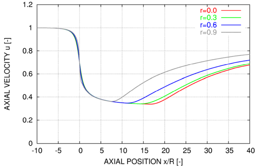
AD simulations -- constant loading CT=0.89
