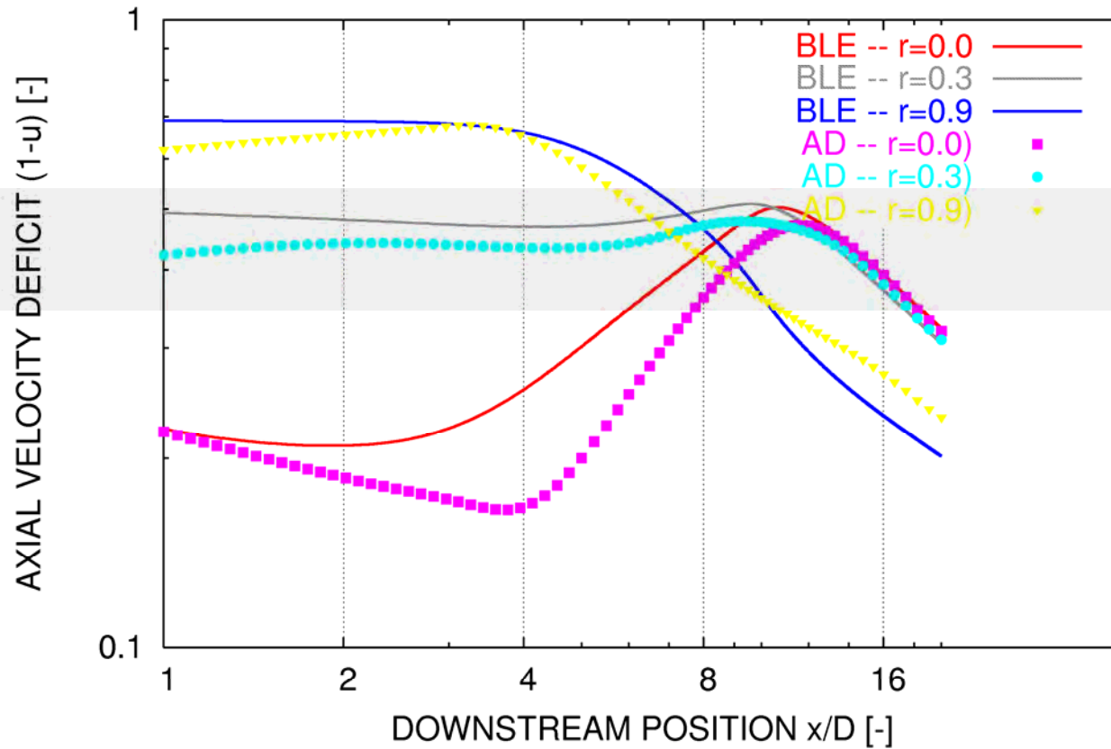
AD and BLE simulations -- NM80 TURBINE -- 6m/s
