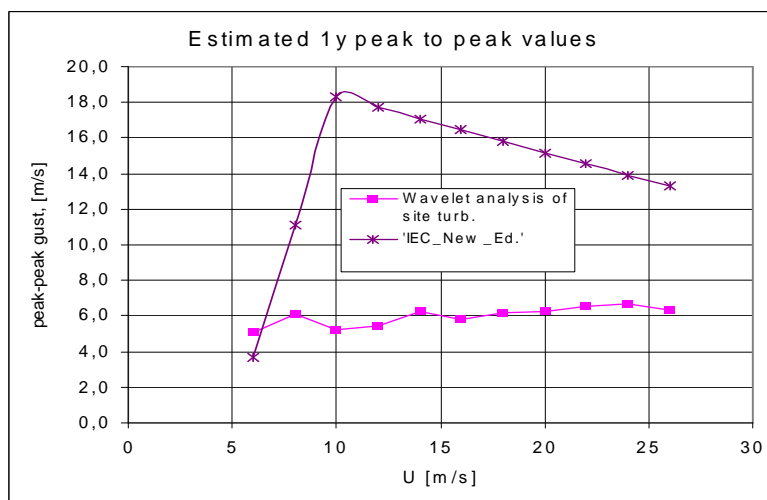
Figure 1: Most likely extreme gust amplitudes as function of the wind speed.
