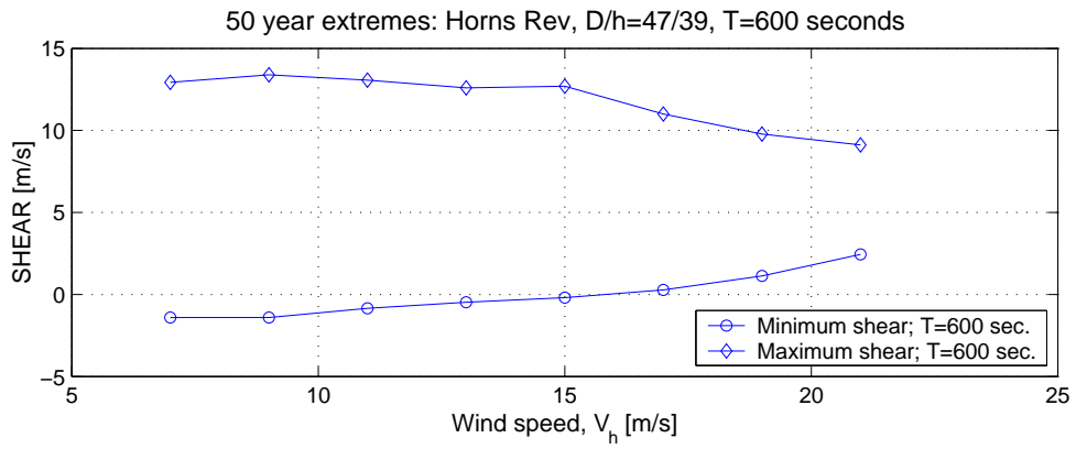
Figure 8: 50-years extreme wind shear at Horns Rev, D/h=47/39, T=600 seconds.
