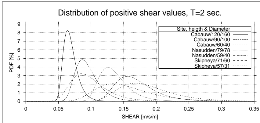
Figure 3b : Distribution of positive shear values.
