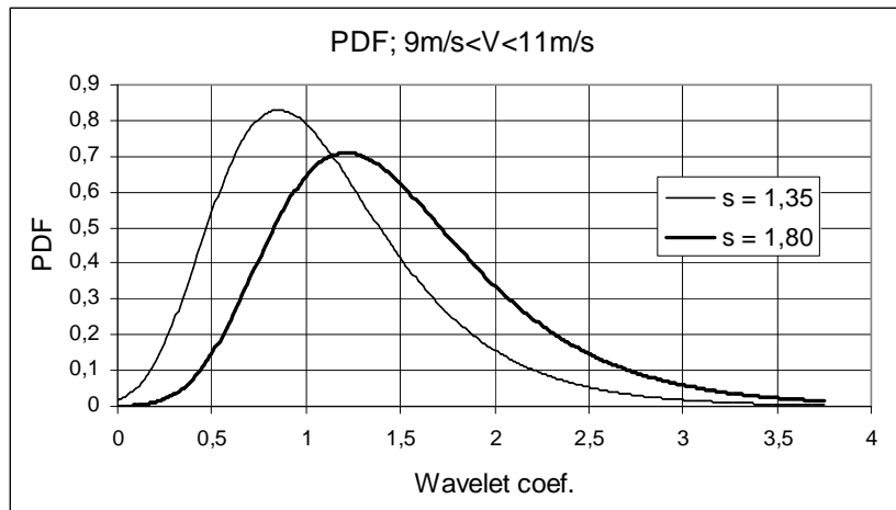
Figure 3: PDF of extreme wavelet coefficients with scales s_{50} and s_I , respectively.
